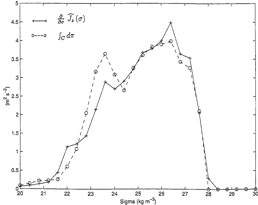
FIG. 8. Annual average of \partial \hat{J}_z(\sigma)/\partial \sigma as a function of \sigma (solid line) and annual average of \int_C d\pi as a function of \sigma (dotted line).
