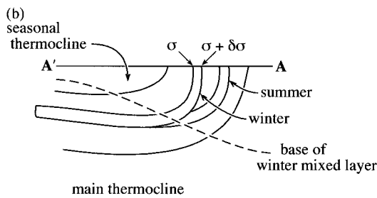
FIG. 2. (a) Schematic plan view of the outcrop window \sigma \rightarrow \sigma + \delta\sigma , and the reference outcrop \sigma_1 ; (b) vertical section showing the same isopycnal layer.
