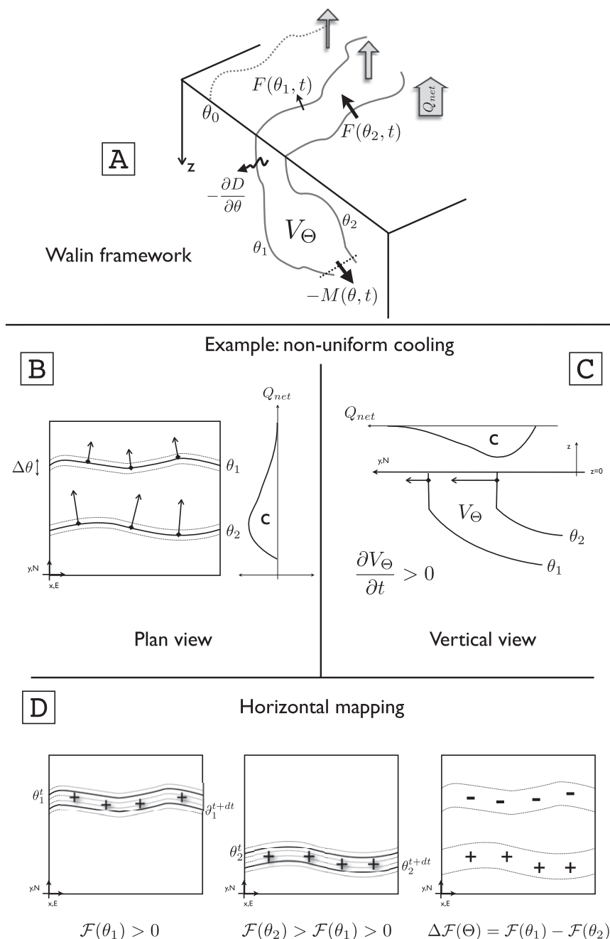
FIG. 2. (a) Schematic of the control volume bounded by isotherms \theta_1 and \theta_2 , which is the subject of Walin's (1982) theoretical framework: V_\Theta is the volume of the layer \Theta , F and \partial_\theta D are the surface and internal diathermal volume flux components, M(\Theta) is the flow out of the control volume, and the vertical gray arrows represent air-sea fluxes. Temperature \theta_0 labels a reference surface. (b)–(c) Horizontal and vertical views of the two isotherms bounding the \Theta layer with a nonuniform meridional profile of heat flux cooling ("c"). Black arrows represent the diathermal volume flux across isotherms. (d) Maps (from the left to the right) of transformation rates across \theta_1 , \theta_2 , and formation rate of the \Theta layer, time-integrated between t and t + dt . The thick contours correspond to consecutive isotherm positions (thin contours demarcate associated temperature classes) and positive (negative) signs denote areas of positive (negative) rates.
