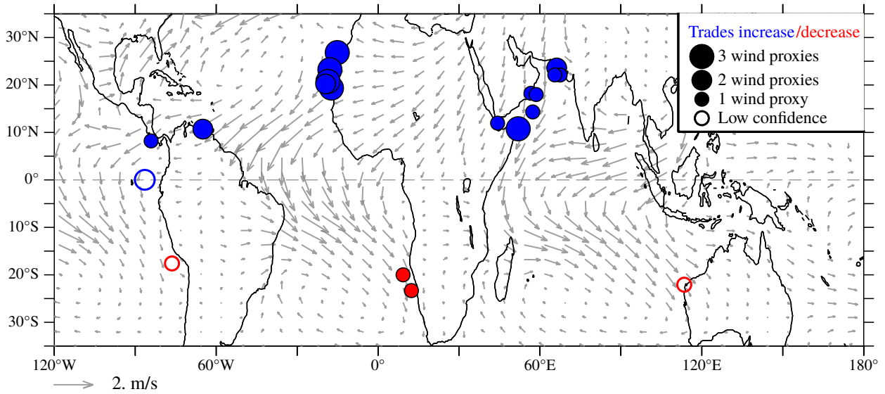
565 Figure 5. Map of proxy inferences of trade wind changes during Heinrich stadials on top of map of annually averaged near-surface wind anomalies (10 m) from the CM2Mc hosing experiment, from Figure 2A. Blue: implied increase in trade wind strength. Red: implied decrease in trade wind strength. Symbol size indicates the number of trade wind proxies (e.g., SSTs, productivity, dust flux) available at each site. Empty symbols indicate records with insufficient chronological 570 control or temporal resolution or with questions as to their interpretation. Some symbols have been slightly displaced to make them visible on the map.
