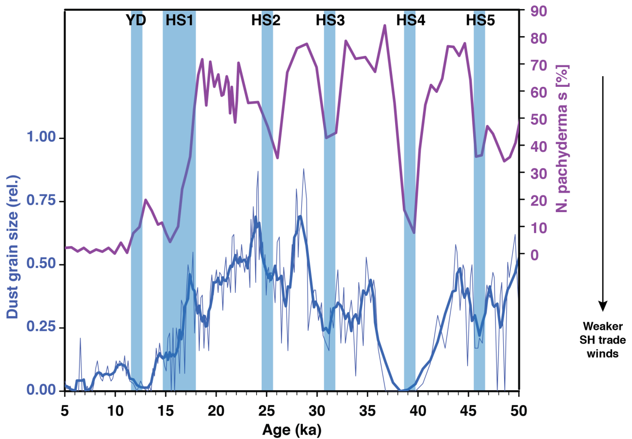
Figure 4. Trade wind proxies from the South Atlantic showing evidence for trade wind weakening in association with southward ITCZ shifts during Heinrich stadials of the last 50 ka.
