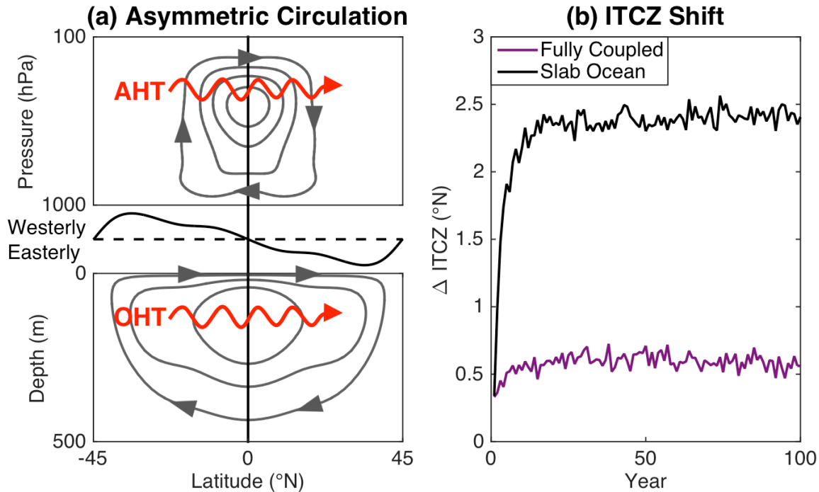
615 Figure 6. The tropical atmosphere and ocean response to NH cooling. A. Anomalies in zonal mean, annual mean atmospheric and shallow ocean circulation in response NH cooling. Top panel shows anomalies in Hadley circulation; middle panel shows changes in zonal component of near-surface winds, showing strengthening of easterly winds in the NH and weakening in the SH; bottom panel shows resulting shallow ocean circulation anomalies. The anomalous 620 atmospheric and ocean circulations both act to transport heat into the NH (thick arrows). Contours indicate stream function anomalies. B. ITCZ shifts in response to cooling of one hemisphere in idealized climate model simulations. The black line shows a large ITCZ shift toward the warmer hemisphere in an uncoupled “slab” ocean simulation. The purple line shows a much smaller ITCZ shift in response to the same perturbation in a coupled simulation; the 625 smaller response is primarily due to heat transport associated with the anomalous tropical ocean circulation shown in panel A. Note that the cooling perturbation and ITCZ responses in this simulation are not meant to resemble those during a Heinrich stadial, only to demonstrate the
