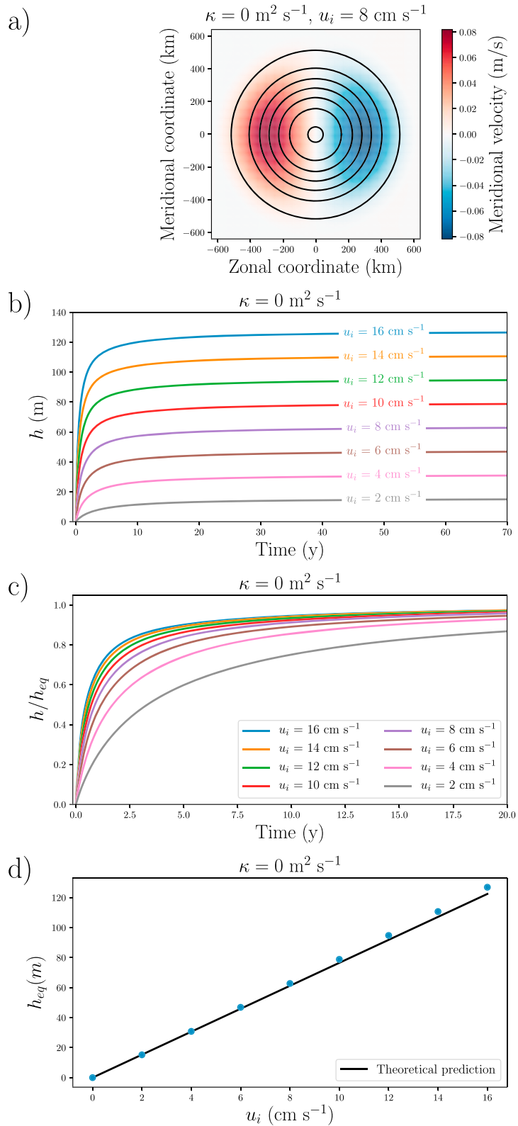
Figure 4. (a) Eulerian-mean meridional velocity (colors) and layer thickness (contours, with a contour interval of 10 m) from the final 10 years of the \kappa = 0 \text{ m}^2 \text{ s}^{-1} u_i = 8 \text{ cm/s} simulation. (b) Temporal evolution of the isopycnal depth anomaly for a range of imposed ice velocities with the thickness diffusivity, \kappa , set to 0. (c) The normalized isopycnal depth anomaly shows that the adjustment timescale depends on u_i . (d) Equilibrium isopycnal depth anomaly plotted against u_i (dots), with the prediction from equation (7) using the values from Table 1 and \alpha = 1 shown by the black line.
