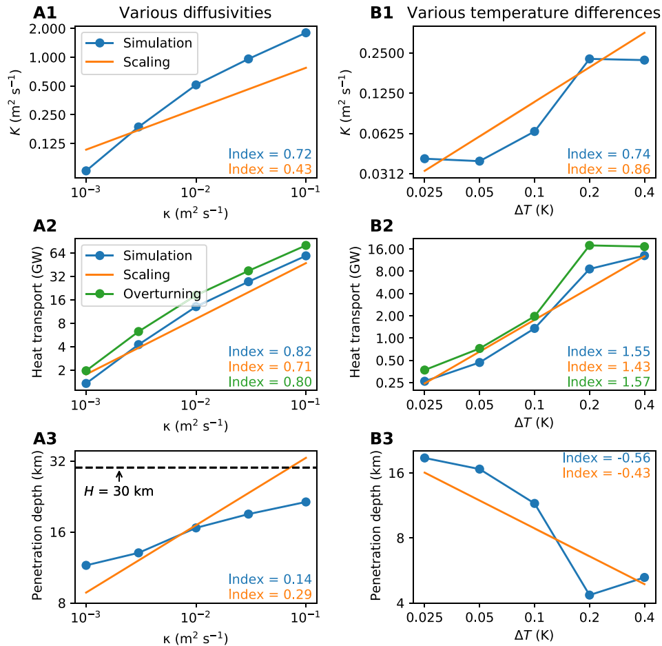
Fig. 6. Measures of key flow parameters in two groups of simulations compared to predictions from scaling. The left column shows the (A1) eddy heat transport coefficient K , (A2) meridional heat transport, and (A3) penetration depth in calculations in which the vertical diffusivity, \kappa , is varied; the right column (B1 to B3) shows the same but when the prescribed temperature difference is varied. Theoretical predictions are made from Eqs. 23, 24, and 25. The overturning [green lines in (A2) and (B2)] represents the meridional heat transport calculated from streamfunction (Eq. 9). The index for the best power fit for each curve is shown in every panel with the corresponding color.
