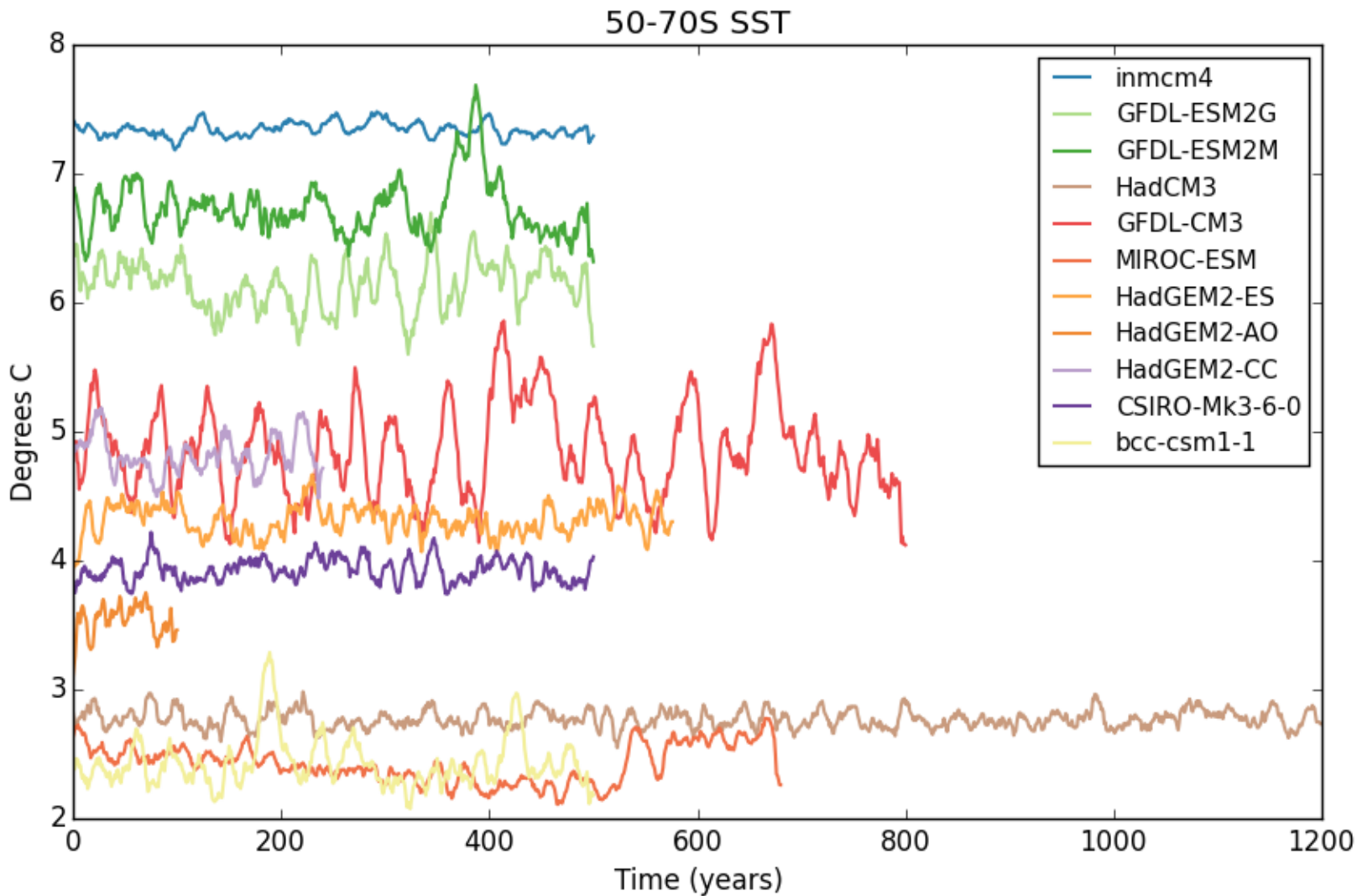
Figure 2: De-trended DJF 50-70°S SSTs for various CMIP5 Models with a 10-year smooth
