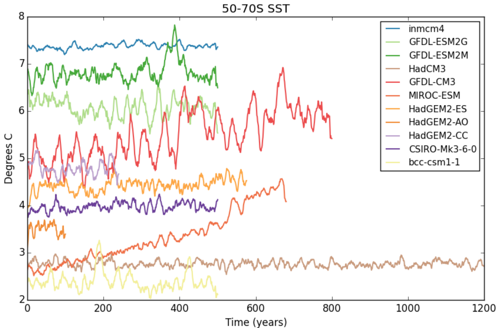
Figure 1: DJF 50-70°S SSTs for various CMIP5 Models with a 10-year smooth.
