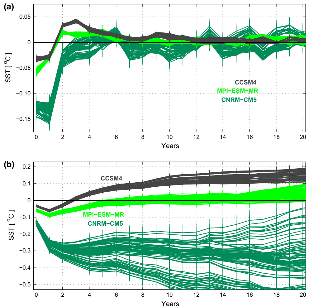
Fig. 4 Annual-mean response of the Southern Ocean SST anomaly [°C] to: a a positive impulse perturbation in the SAM index of magnitude equal to \overline{\sigma_{SAM}^{Ens}} , b a positive step increase in the SAM index of magnitude equal to \overline{\sigma_{SAM}^{Ens}} . Different colors are used to distinguish the response functions in the three CMIP5 models shown: CCSM4, MPI-ESM-MR, and CNRM-CM5. For each model, we have shown only 100 different fits to illustrate the envelopes of uncertainty, and we have not spanned the full parameter space laid out in Table 2. Vertical error bars denote the margin of error for each fit
